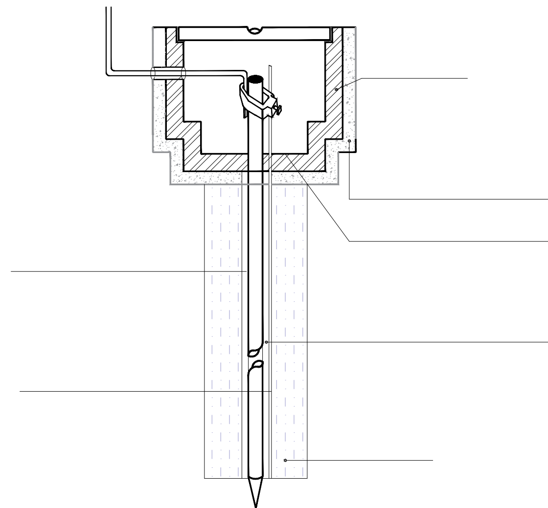
TYPICAL DETAIL OF ROD EARTHING
